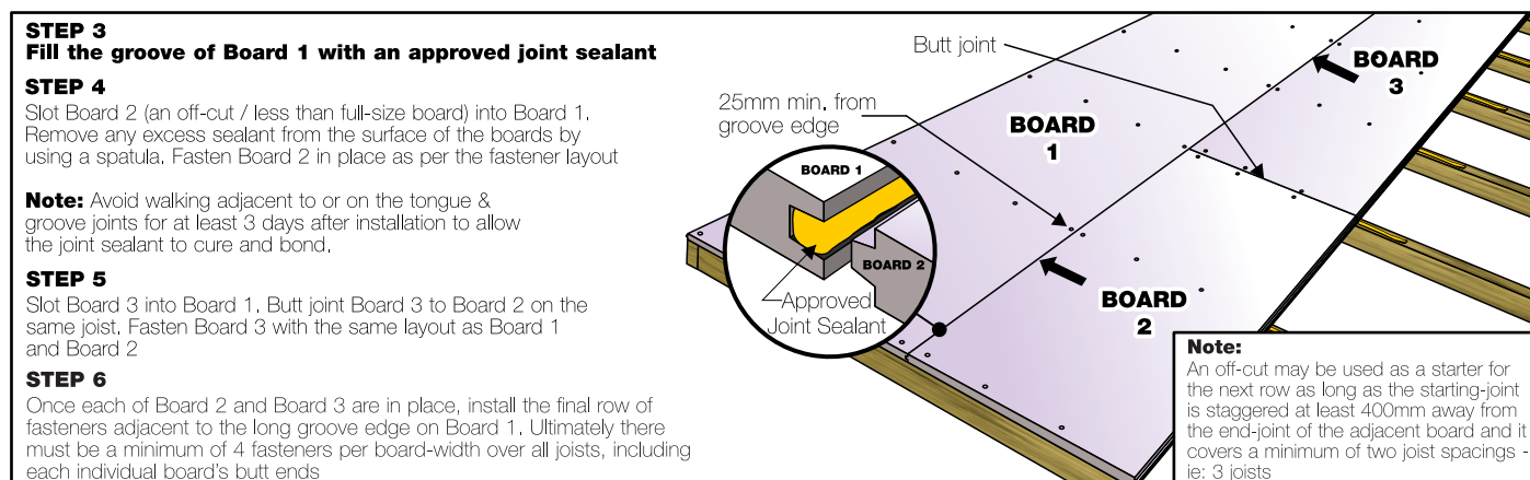
FIGURE 6 – FIXING SECOND AND THIRD BOARDS
